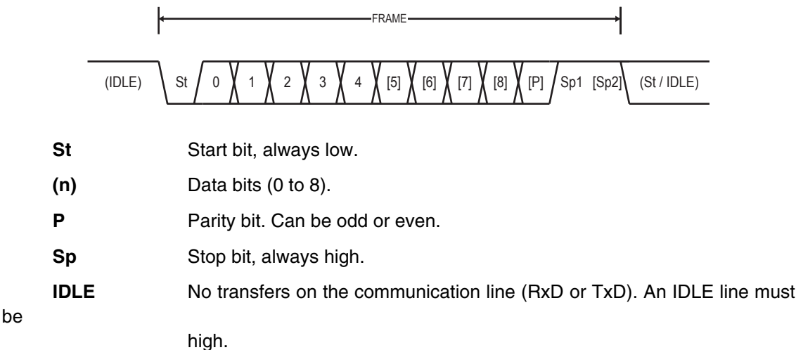
Figure 20-4. Frame Formats
