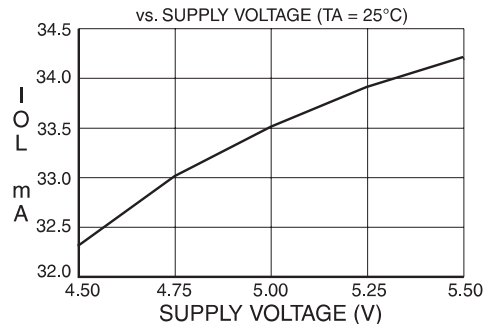
OUTPUT SINK CURRENT vs. SUPPLY VOLTAGE (TA=25°C)
