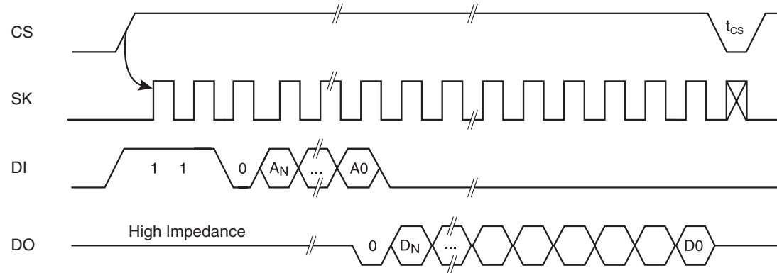
Figure 5-2. READ Timing
