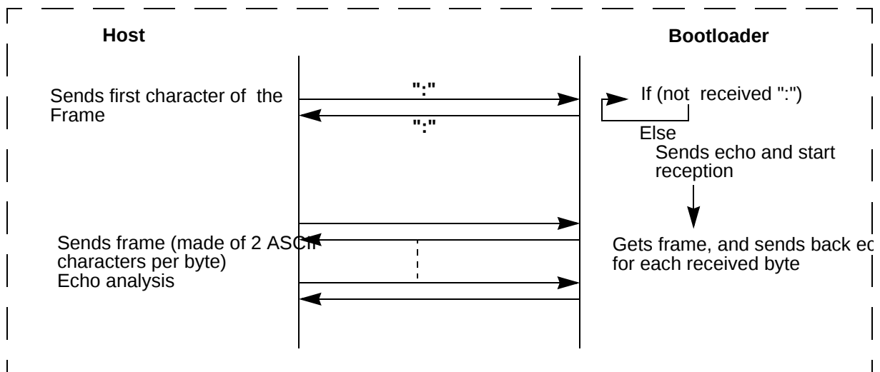
Figure 52. Command Flow
