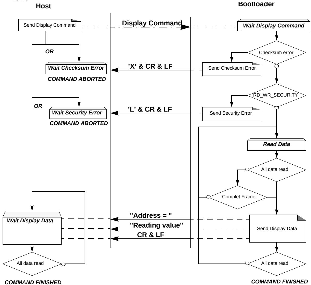
Figure 55. Display Flow
