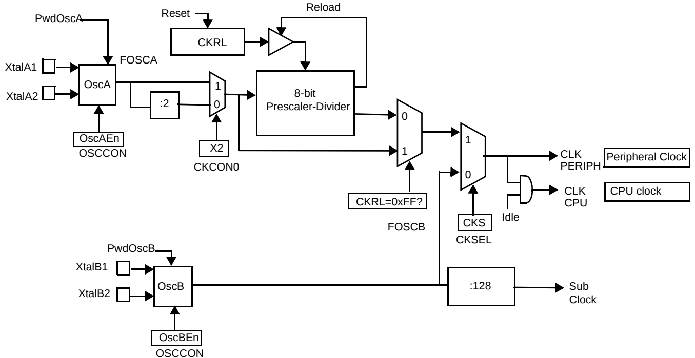
Figure 2. Functional Oscillator Block Diagram
