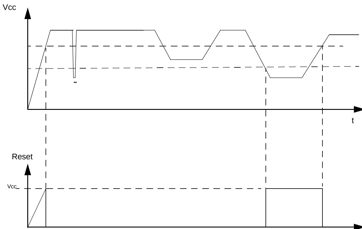
Figure 11. Power Fail Detect
