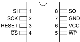
Figure 2-2. 8-SOIC
