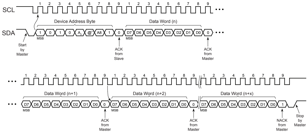
Figure 8-3. Sequential Read
