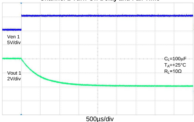
Channel 1 Turn-Off Delay and Fall Time
