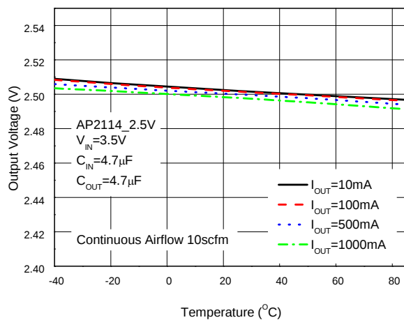
Figure 18. Output Voltage vs. Temperature
