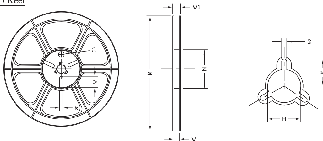
QFN5x5 Reel
