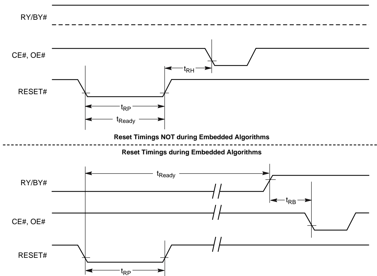
Figure 17. RESET# Timings
