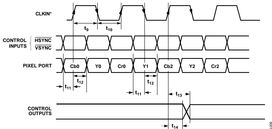
Figure 8. ED/HD-DDR Input, 8-/10-Bit 4:2:2 YCrCb ( \overline{\text{HSYNC}}/\overline{\text{VSYNC}} ), Input Mode 010
