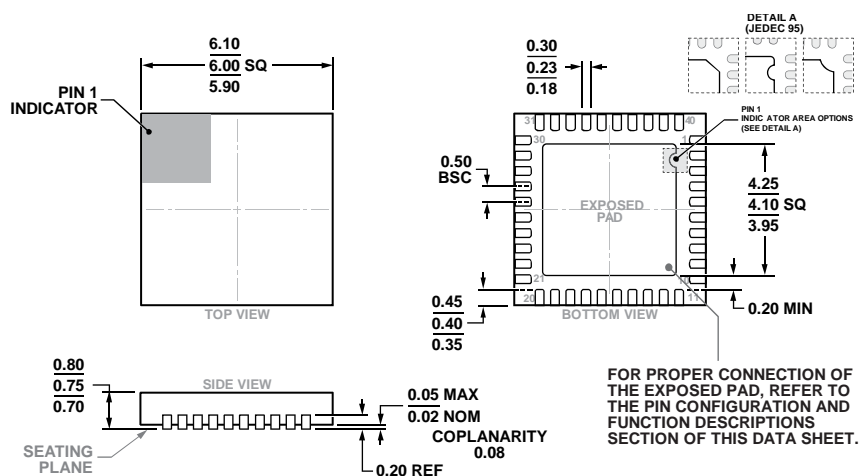
Figure 148. 40-Lead Lead Frame Chip Scale Package [LF CSP] 6 mm × 6 mm Body and 0.75 mm Package Height (CP-40-9) Dimensions shown in millimeters
