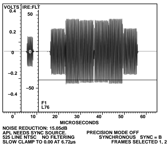
Figure 134. NTSC Chroma
