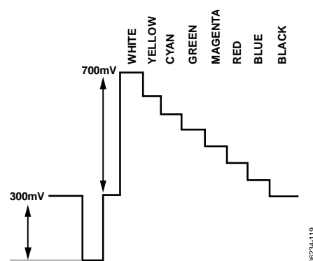
Figure 121. Y Levels—PAL
