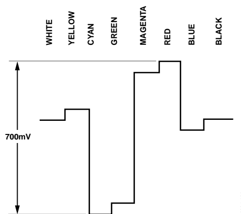
Figure 122. Pr Levels—PAL
