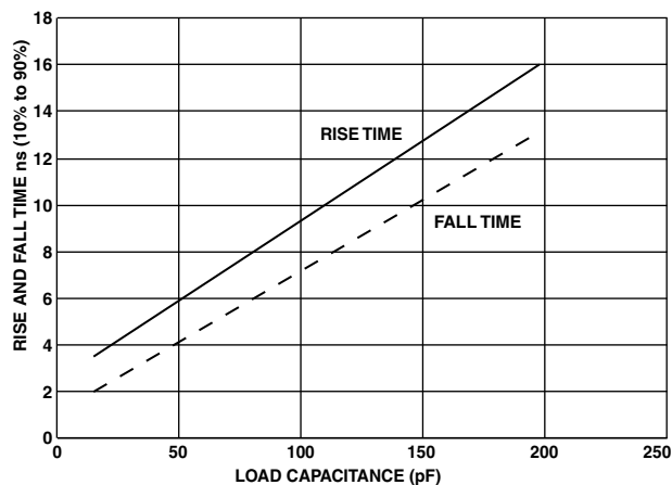
Figure 58. Typical Rise and Fall Times (10% to 90%) vs. Load Capacitance for Driver D at V_{DDEXT} = 2.25V
