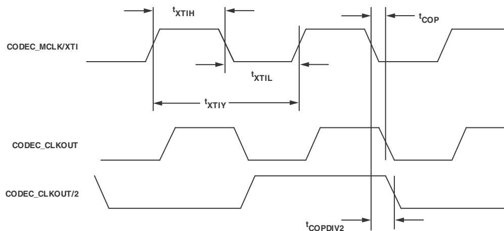
Figure 22. System (CODEC_MCLK) Clock Timing
