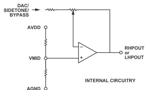
Figure 5. Headphone Output
