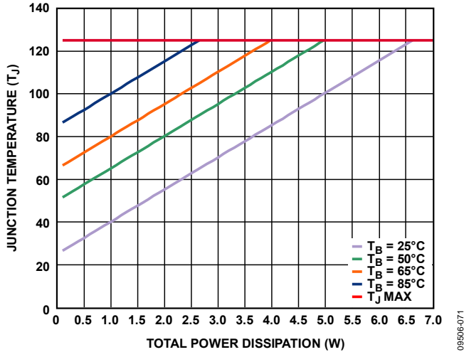
Figure 76. LFCSP
