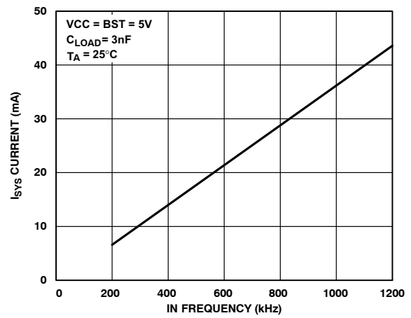
Figure 14. Supply Current vs. Frequency
