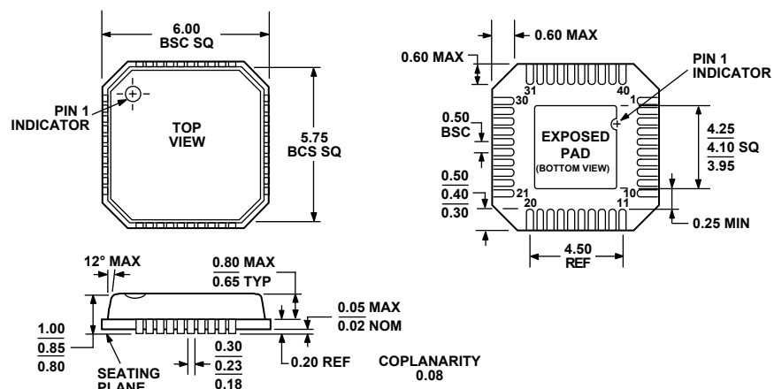
COMPLIANT TO JEDEC STANDARDS MO-220-VJJD-2 Figure 20. 40-Lead Lead Frame Chip Scale Package [LFCSP_VQ] 6 mm × 6 mm Body, Very Thin Quad (CP-40) Dimensions shown in millimeters
