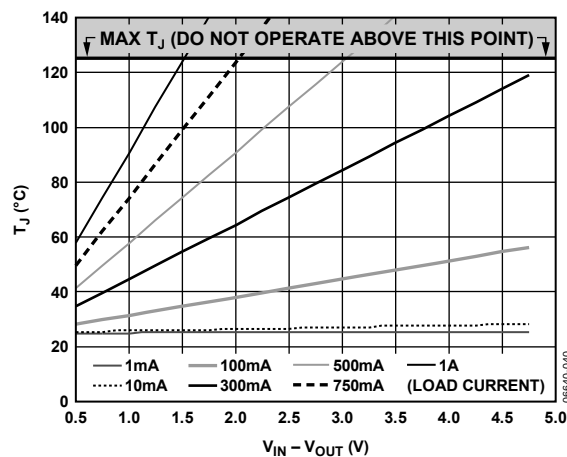
Figure 41. 0 mm² of PCB Copper, T_A = 25^\circ\text{C} , LFCSP
