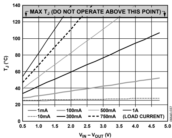
Figure 38. 0 mm² of PCB Copper, T_A = 25^\circ\text{C} , SOIC
