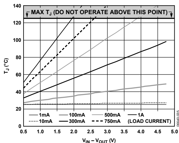
Figure 36. 500 mm² of PCB Copper, T_A = 25^\circ\text{C} , SOIC
