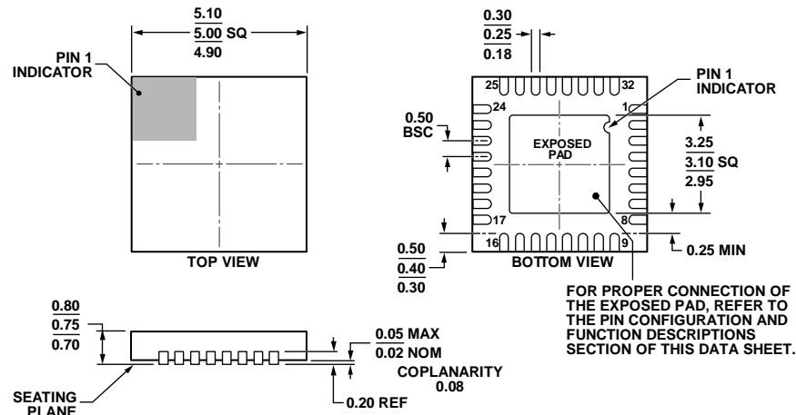
Figure 62. 32-Lead Lead Frame Chip Scale Package [LFCSP_WQ] 5 mm x 5 mm Body, Very Very Thin Quad (CP-32-7) Dimensions shown in millimeters
