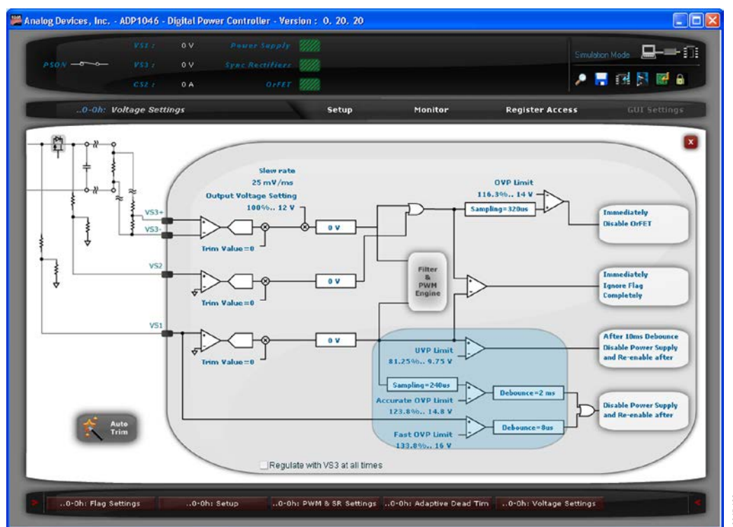
Figure 41. Voltage Sense Window in Simulation Mode (ADP1046 GUI)
