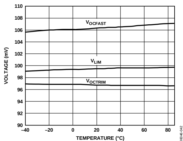
Figure 23. V_OCTRIM, V_LIM, V_OFAST vs. Temperature
