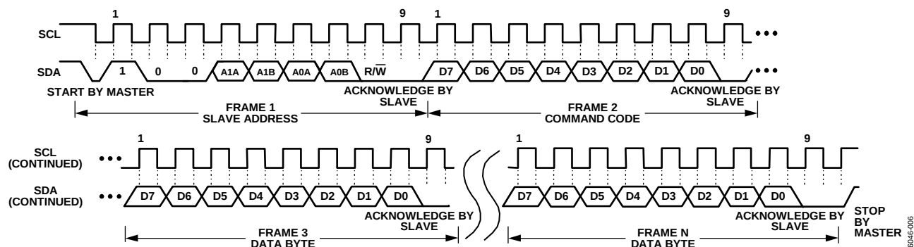
Figure 32. General I²C Write Timing Diagram
