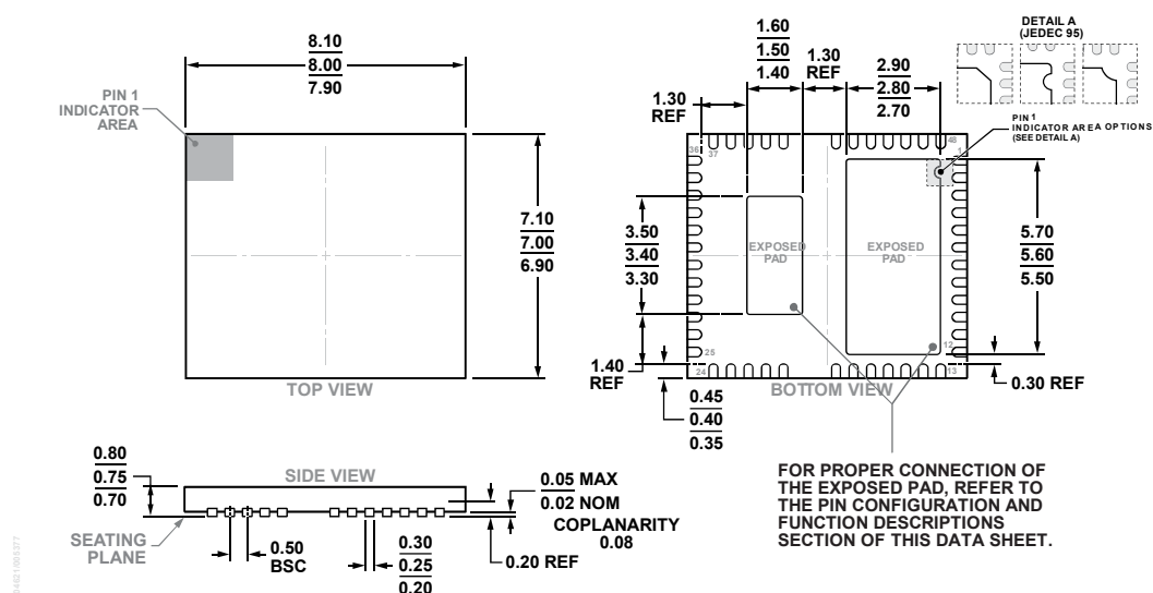
Figure 52. 48-Lead Lead Frame Chip Scale Package [LFCSP] 8 mm x 7 mm Body and 0.75 mm Package Height (CP-48-18) Dimensions shown in millimeters
