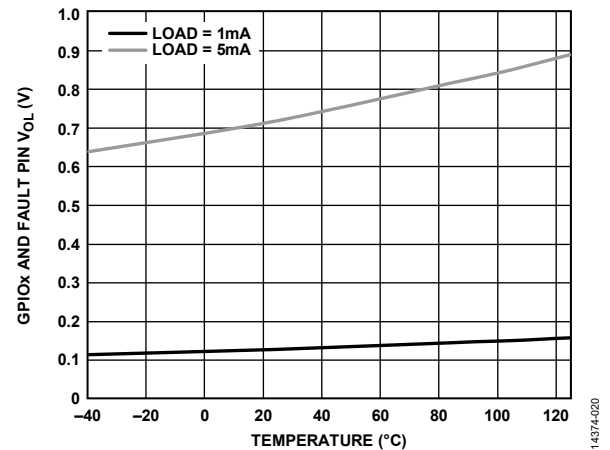
Figure 21. GPIOx and Fault Pin V_{OL} vs. Temperature
