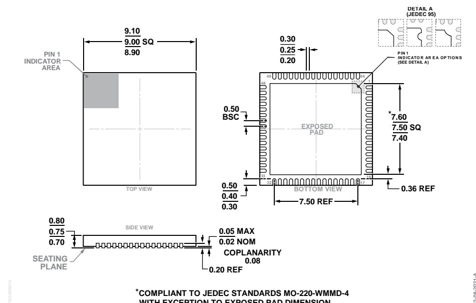
Figure 30. 64-Lead Lead Frame Chip Scale Package [LFCSP] 9 mm x 9 mm Body and 0.75 mm Package Height (CP-64-23)
