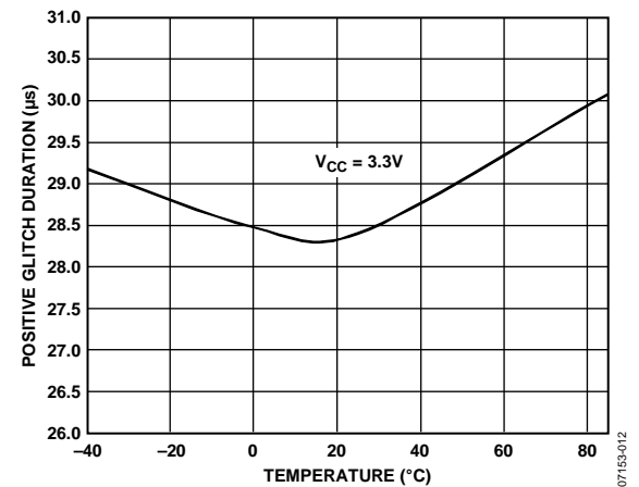
Figure 10. VINx Input Positive Glitch Immunity vs. Temperature
