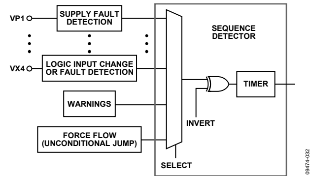
Figure 20. Sequence Detector Block Diagram
