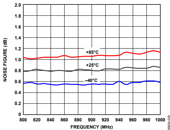
Figure 29. Noise Figure vs. Temperature
