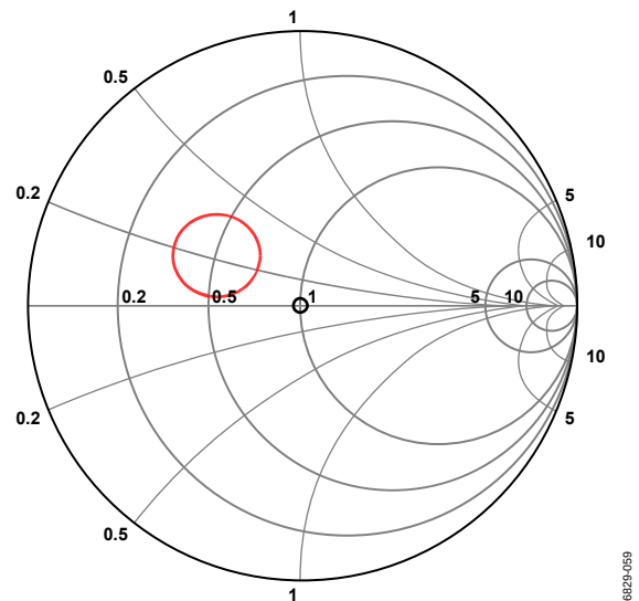
Figure 61. Area of Optimal Noise Matching for ADL5523
