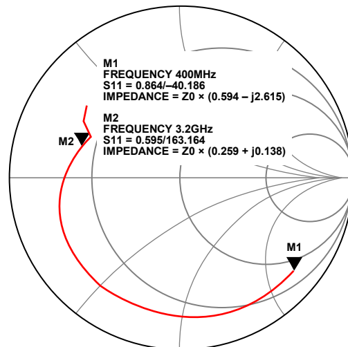
Figure 64. S11 of ADL5523 with S22 Matched at 3.2 GHz
