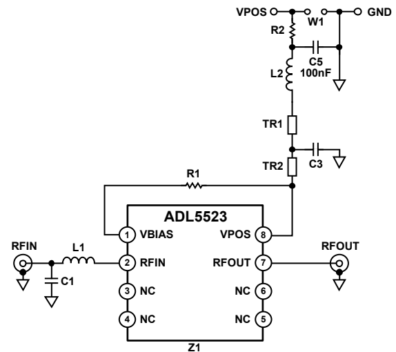
Figure 53. ADL5523 Basic Connections
