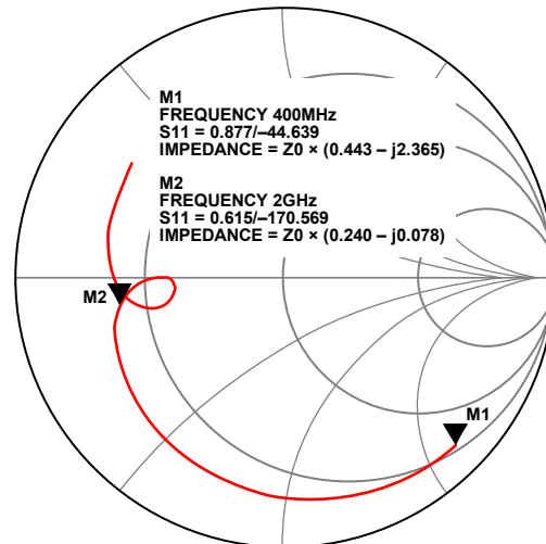
Figure 63. S11 of ADL5523 with S22 Matched at 2 GHz
