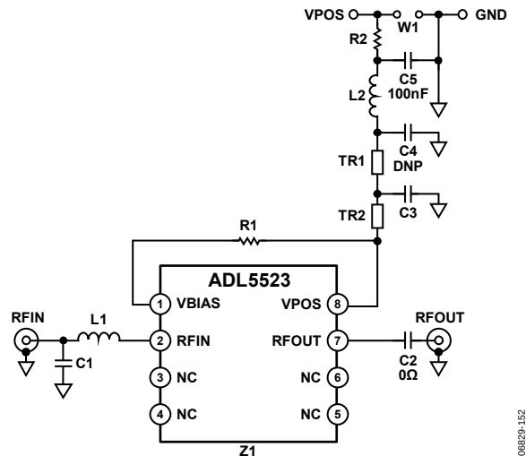
Figure 54. Evaluation Board Schematic
