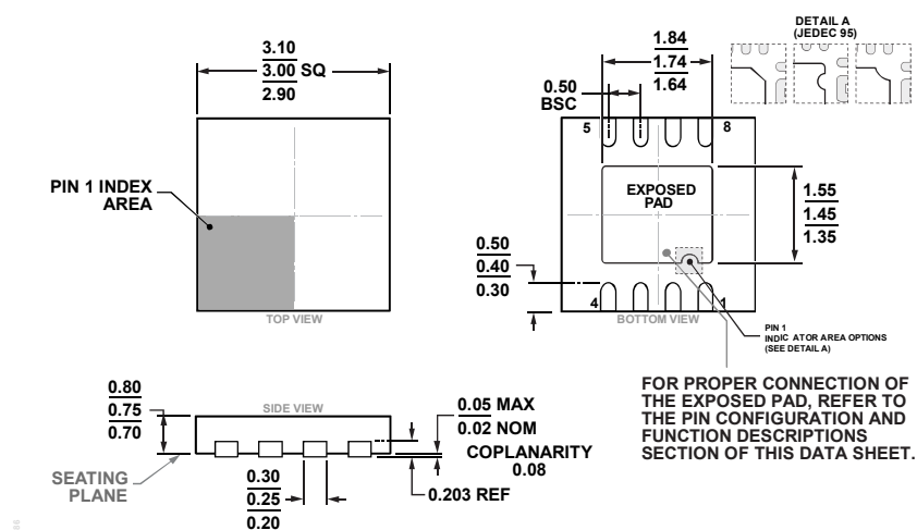
Figure 65. 8-Lead Lead Frame Chip Scale Package [LFCSP] 3 mm × 3 mm Body and 0.75 mm Package Height (CP-8-13)
