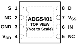
Figure 2. 8-Lead LFCSP Pin Configuration
