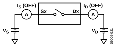
Figure 23. Off Leakage
