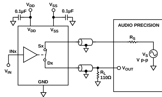
Figure 31. THD + Noise
