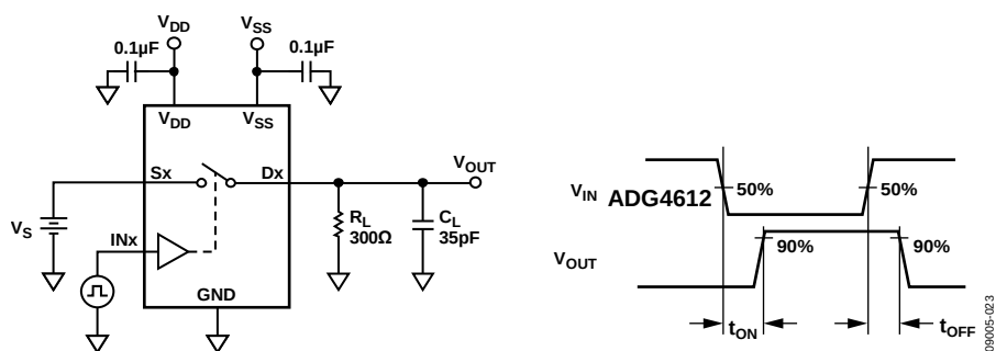
Figure 25. Switching Times
