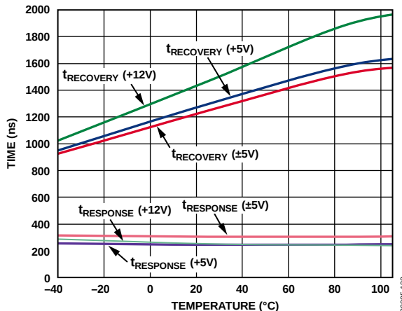
Figure 20. Fault Response Time/Fault Recovery Time
