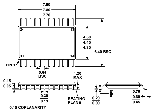
Figure 45. 24-Lead Thin Shrink Small Outline Package [TSSOP] (RU-24) Dimensions shown in millimeters
