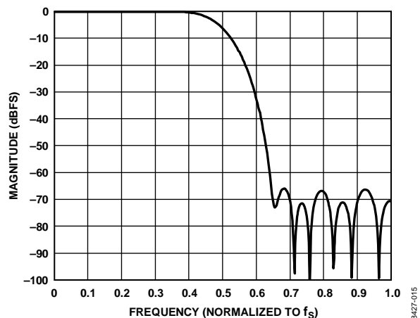
Figure 14. DAC Interpolation Filter, 64x Oversampling, Normalized to f_s
