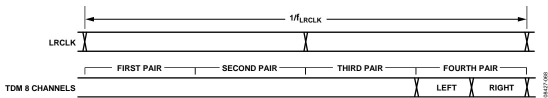
Figure 69. Example of Left Channel First, Fourth Pair TDM Setting
