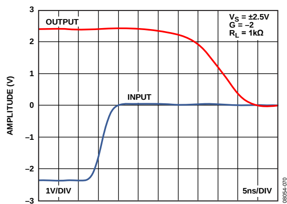
Figure 39. Output Overdrive Recovery from Positive Rail
