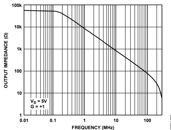
Figure 34. Closed-Loop Output Impedance vs. Frequency, Device Disabled (ADA4891-3 Only)
