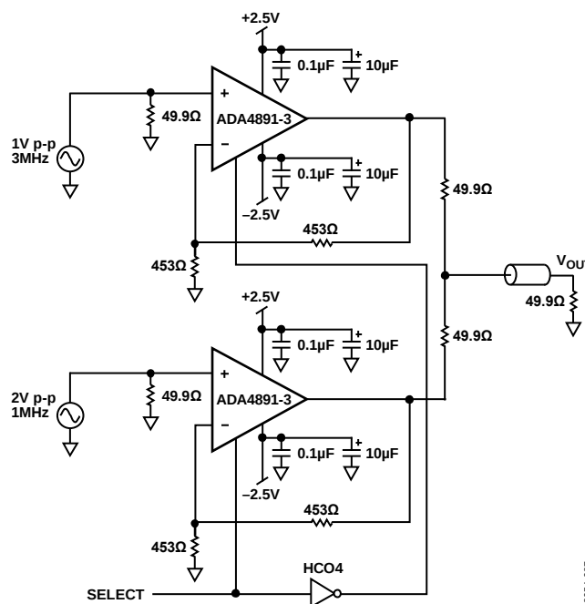
Figure 64. Two-to-One Multiplexer Using Two ADA4891-3 Devices
