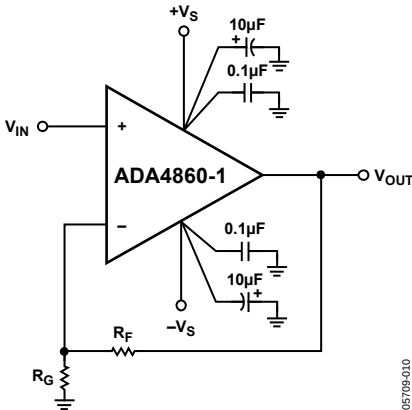
Figure 51. Noninverting Gain
