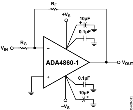
Figure 52. Inverting Gain
