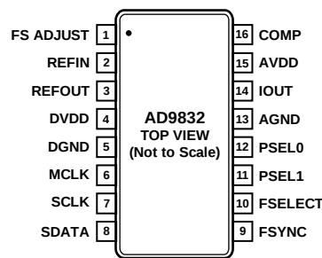
Figure 6. Pin Configuration
