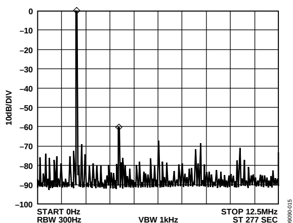
Figure 15. f_{MCLK} = 25 \text{ MHz} , f_{OUT} = 2.1 \text{ MHz} , Frequency Word = 0x15810625
