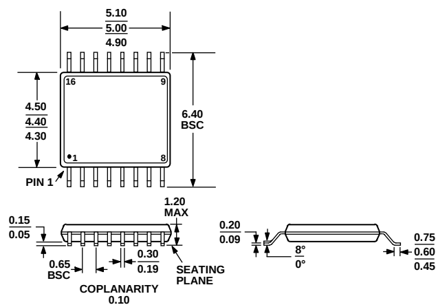
COMPLIANT TO JEDEC STANDARDS MO-153-AB Figure 39. 16-Lead Thin Shrink Small Outline Package [TSSOP] (RU-16) Dimensions shown in millimeters
