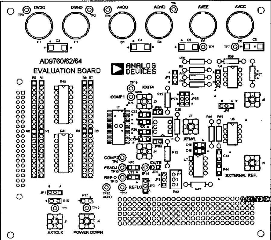
Figure 39. Silkscreen Layer—Top
