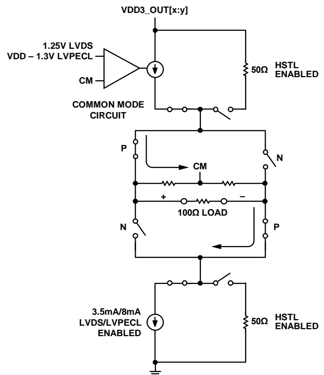
Figure 28. Multimode Driver
