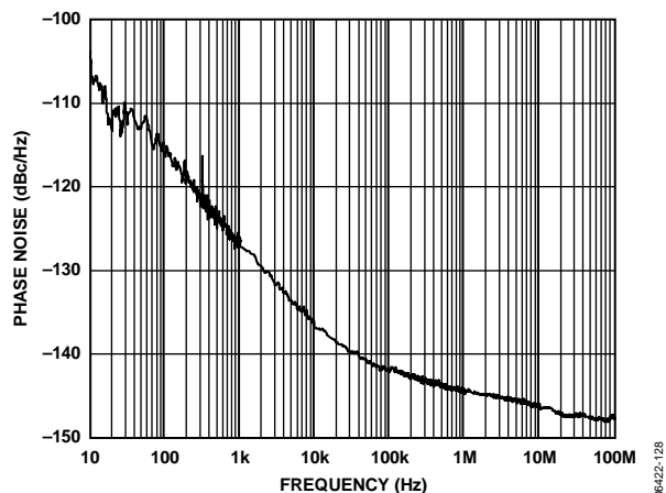
Figure 33. Phase Noise (Additive) LVPECL at 1600 MHz, Divide-by-1
