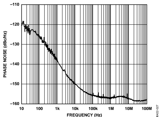
Figure 32. Phase Noise (Additive) LVPECL at 200 MHz, Divide-by-5
