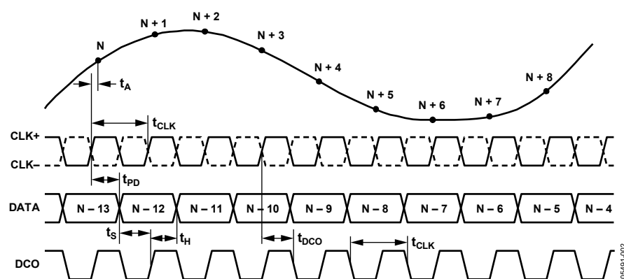
Figure 2. Timing Diagram
