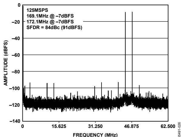
Figure 25. AD9246-125 Two-Tone FFT with f_{IN1} = 169.1 MHz, f_{IN2} = 172.1 MHz
