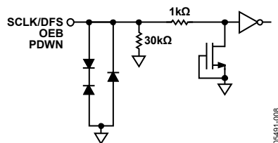
Figure 8. Equivalent SCLK/DFS, OEB, PDWN Input Circuit
