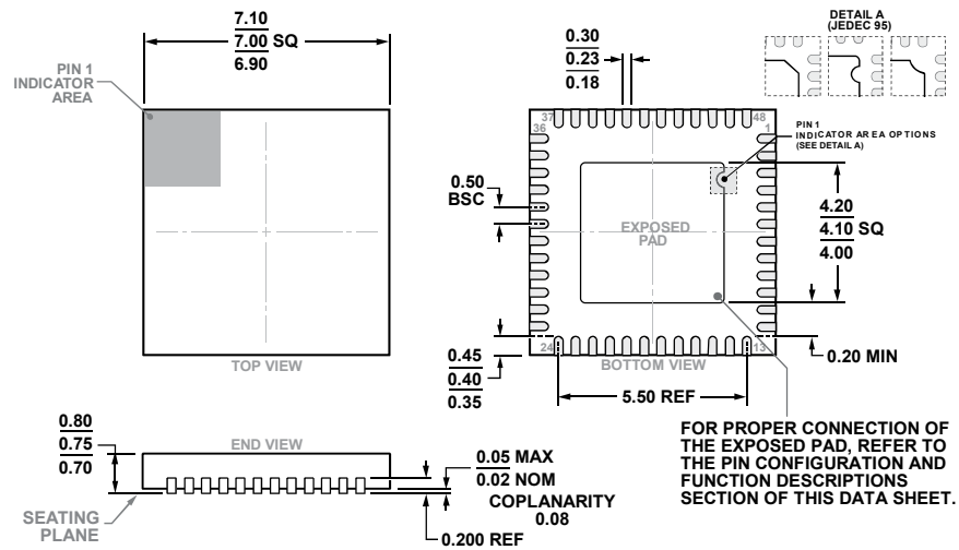
Figure 71. 48-Lead Lead Frame Chip Scale Package [LF CSP] 7 mm × 7 mm Body and 0.75 mm Package Height (CP-48-5) Dimensions shown in millimeters
