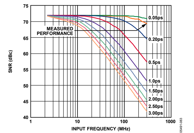
Figure 51. SNR vs. Input Frequency and Jitter
