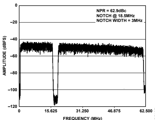
Figure 29. AD9246 Noise Power Ratio (NPR)
