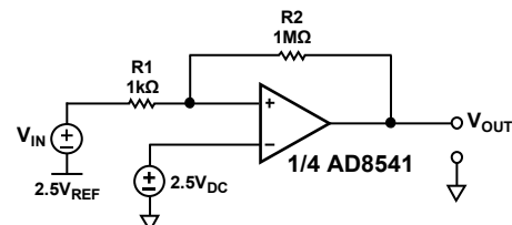
Figure 39. AD854x Comparator Application—Overload Detector
