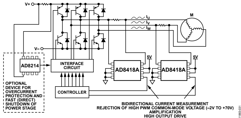
Figure 36. 3-Phase Motor Control
