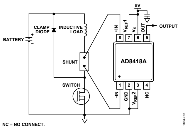
Figure 37. Low-Side Switch
