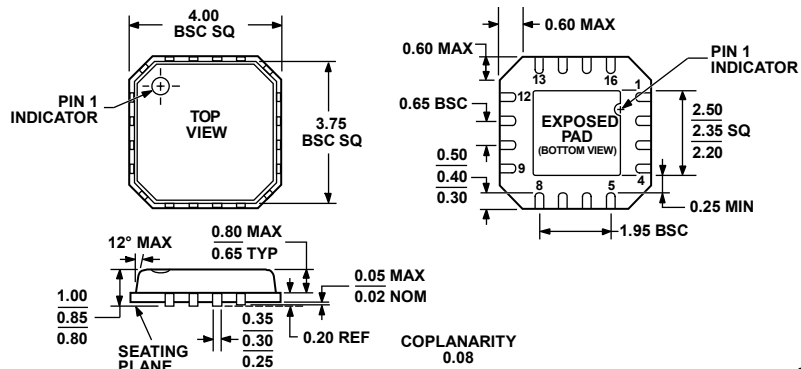
COMPLIANT TO JEDEC STANDARDS MO-220-VGGC Figure 52. 16-Lead Lead Frame Chip Scale Package [LFCSP_VQ] 4 mm × 4 mm Body, Very Thin Quad (CP-16-10) Dimensions are shown in millimeters
