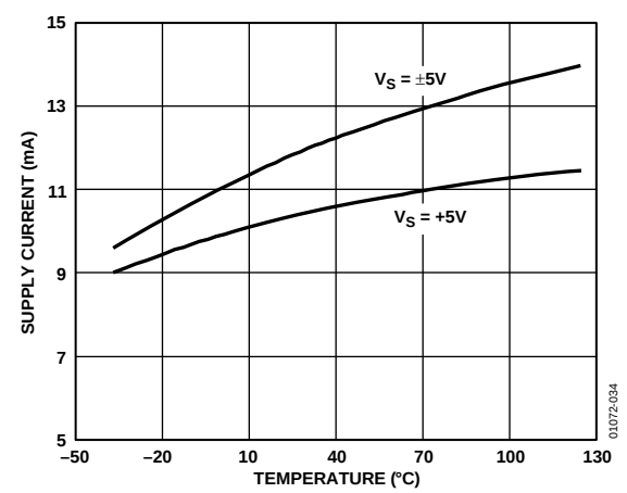
Figure 34. Quiescent Current vs. Temperature
