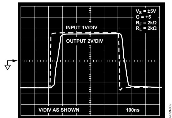
Figure 32. Overdrive Recovery
