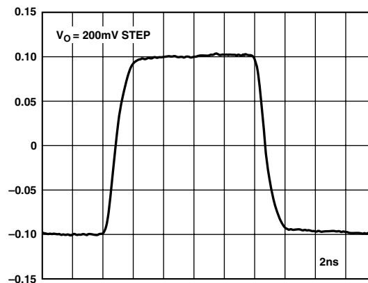
TPC 26. AD8075 Small Signal Pulse Response ( R_L = 150 \text{ k}\Omega )
