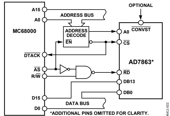
Figure 22. AD7863 to MC68000 Interface
