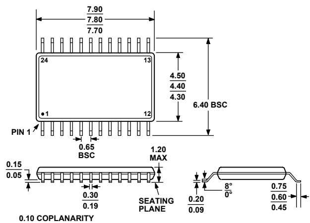
COMPLIANT TO JEDEC STANDARDS MO-153-AD Figure 25. 24-Lead Thin Shrink Small Outline Package [TSSOP] (RU-24) Dimensions shown in millimeters
