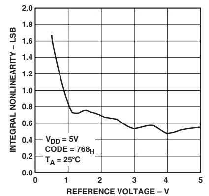
TPC 15. AD7390 INL Error vs. Reference Voltage
