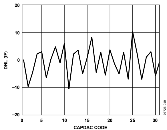
Figure 19. CAPDAC Differential Nonlinearity (DNL), V_{DD} = 1.8\text{ V}
