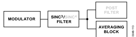
Figure 106. Fast Settling Mode, Sinc 3 + Sinc 1 Filter
