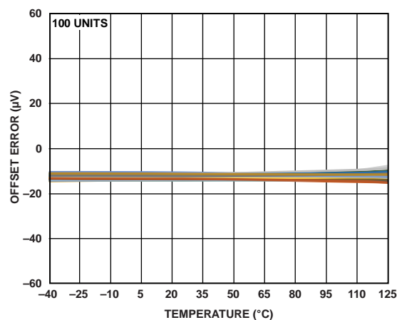
Figure 19. Input Referred Offset Error vs. Temperature (Gain = 16, Full Power Mode)
