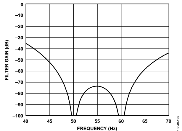
Figure 118. Zoom in 40 Hz to 70 Hz, 20 SPS Output Data Rate, 50 ms Settling Time
