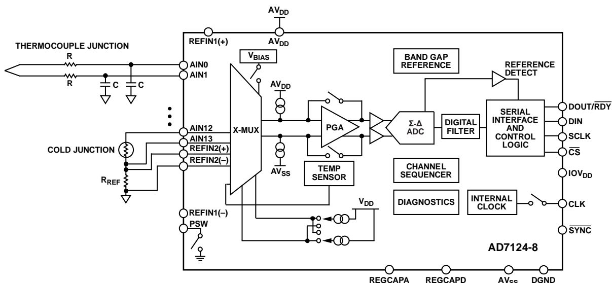
Figure 129. Thermocouple Application
