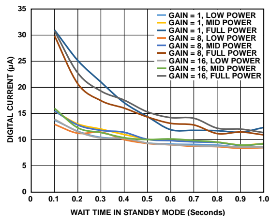
Figure 61. Digital Current vs. Wait Time in Standby Mode, ADC in Single Conversion Mode (50 SPS)
