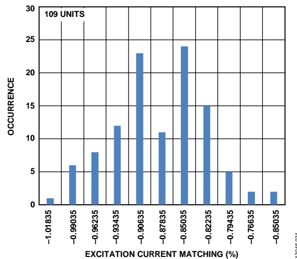
Figure 31. IOUTx Current Initial Matching Histogram (500 \mu A)
