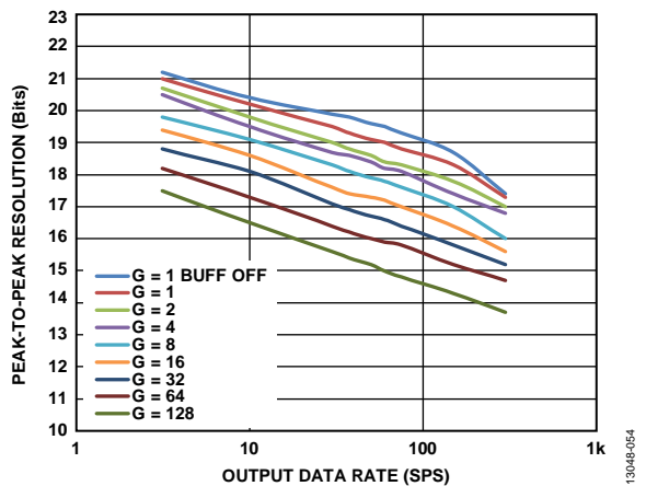
Figure 54. Peak-to-Peak Resolution vs. Output Data Rate (Settled), \text{Sinc}^4 + \text{Sinc}^1 Filter (Mid Power Mode)
