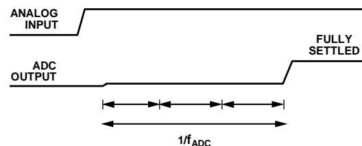
Figure 95. Sinc 3 Zero Latency Operation
