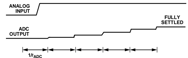
Figure 86. Asynchronous Step Change in the Analog Input
