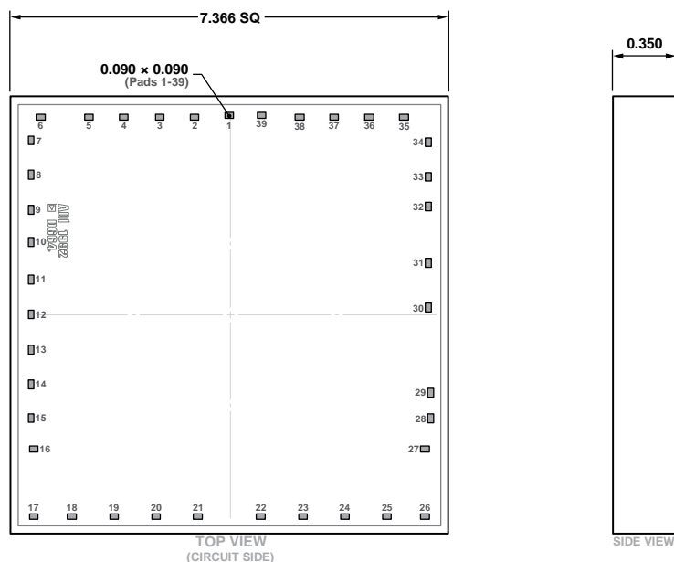
Figure 47. 39-Pad Bare Die [Chip] (C-39-2)
