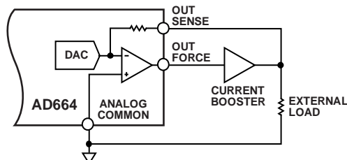
Figure 9. Current Boosting Scheme
