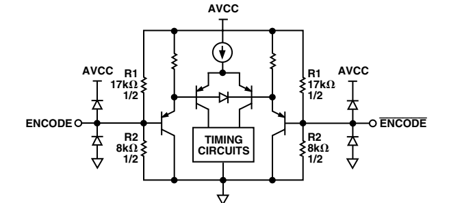
Figure 6. Encode Inputs
