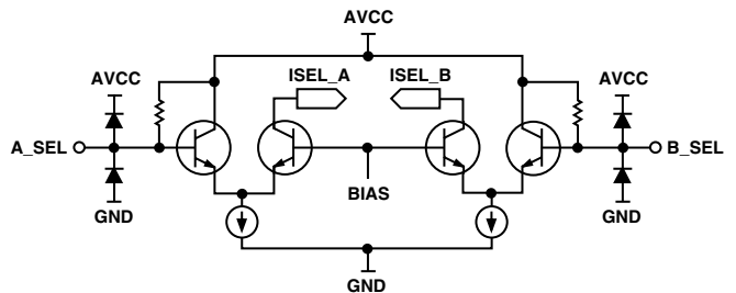
Figure 3. A_SEL, B_SEL Input Mode Pins
