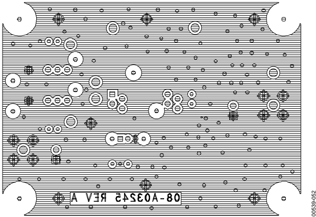
Figure 53. Secondary Side Copper
