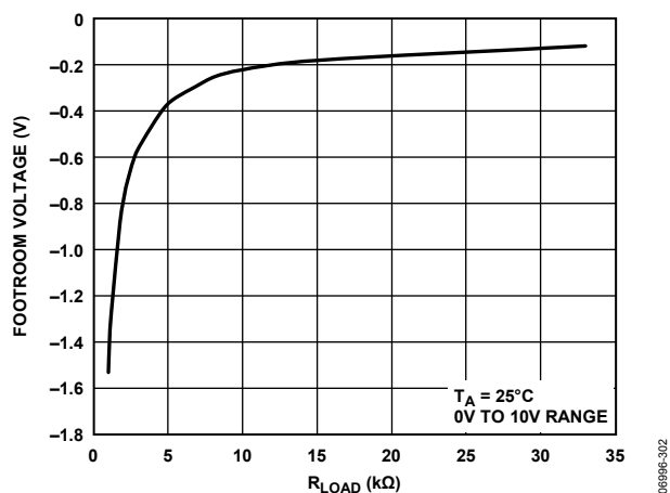
Figure 35. V_{out} Footroom
