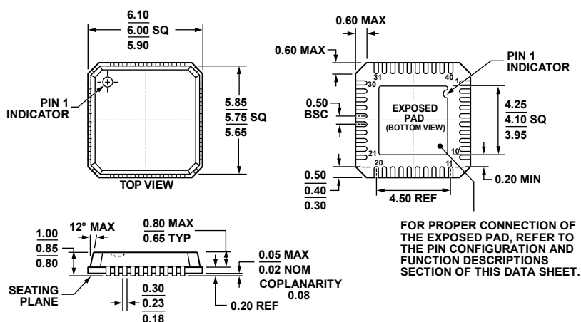
Figure 85. 40-Lead Lead Frame Chip Scale Package [LFCSP] 6 mm × 6 mm Body and 0.85 mm Package Height (CP-40-1)
